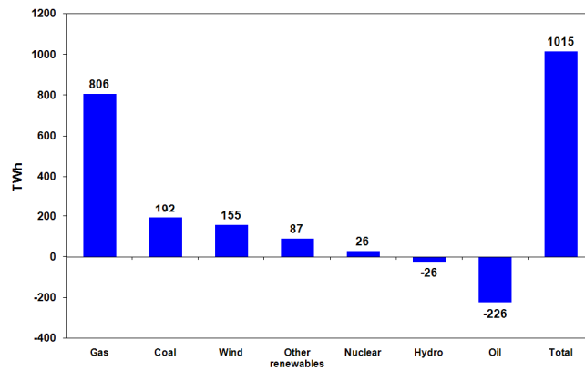
Incremental electricity generated in OECD Countries 2000-08
